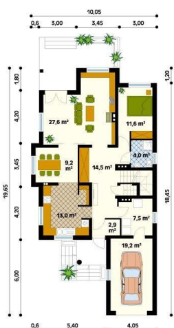
Parter
