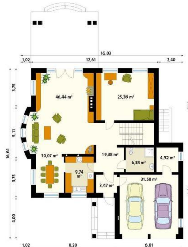
Parter
