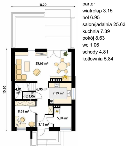
Parter
