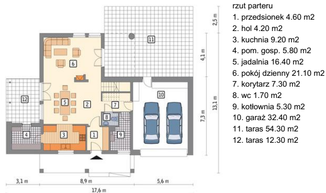
Parter
