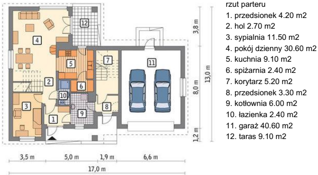
Parter
