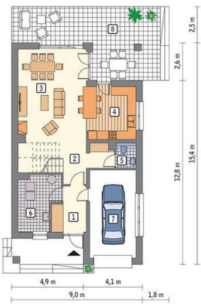
Parter
