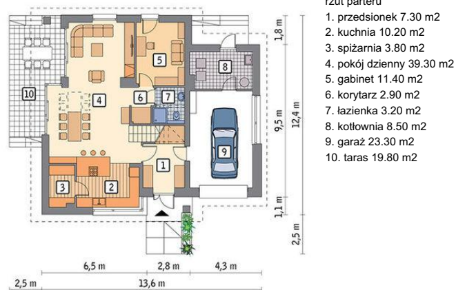
Parter
