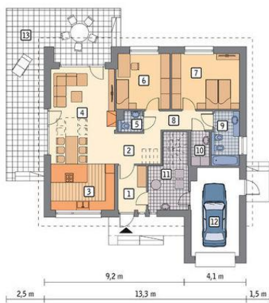
Parter
