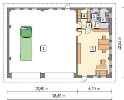
Parter
