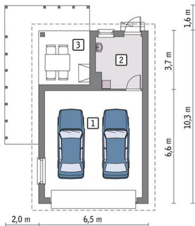
Parter
