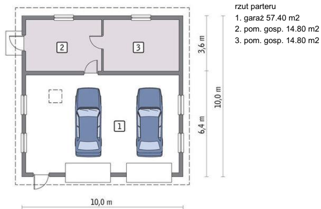
Parter
