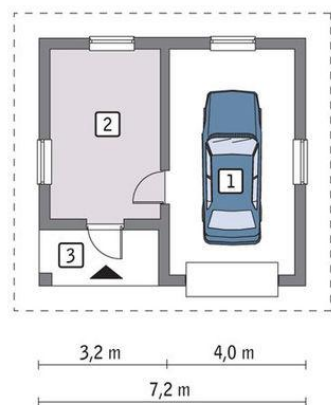
Parter
