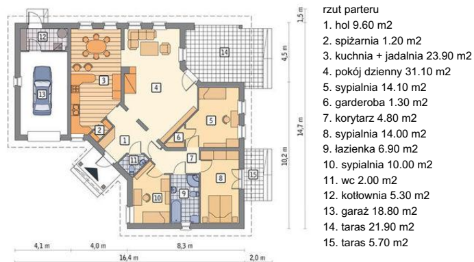
Parter
