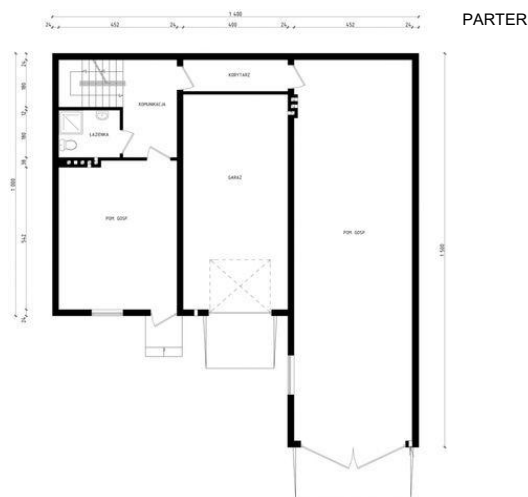
Parter
