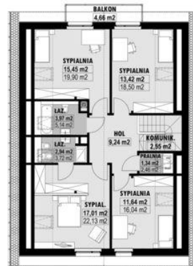
E-257 PODDASZE
