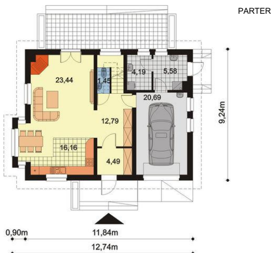
Parter
