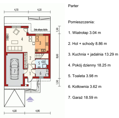
Parter
