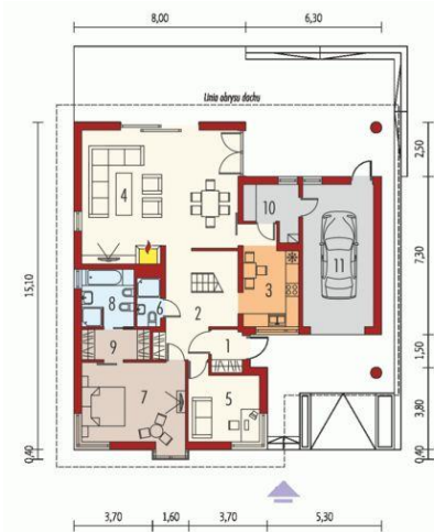
Parter
